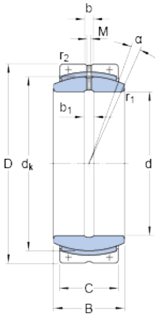
GEC 500 FBAS Bearing 2D drawings and 3D CAD models
